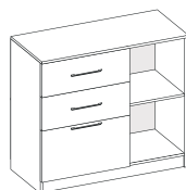
комод-2 1000x910x430
