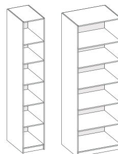
шкаф-4 400/800x2400x584/600
